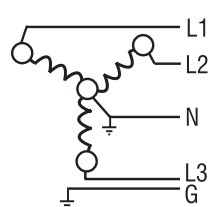
3 Phase Wye 4 Wire + Ground
