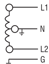
Split Phase 3 Wire + Ground
