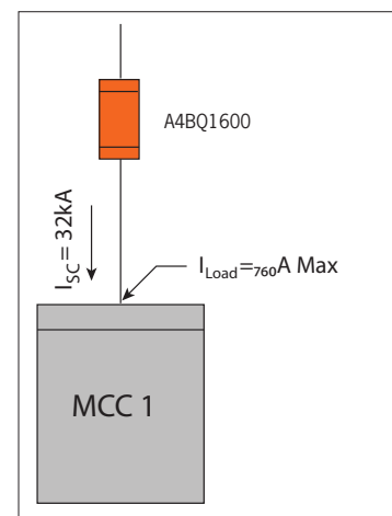
Figure 3: Single Line Diagram
