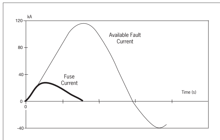
Figure 1. Fuse Current Limitation
