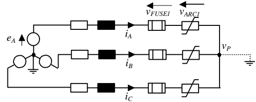
Figure 4. Circuit model
