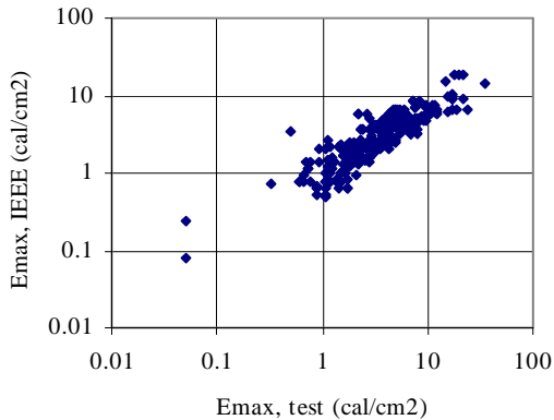
Figure 15. IEEE formula prediction compared with test
