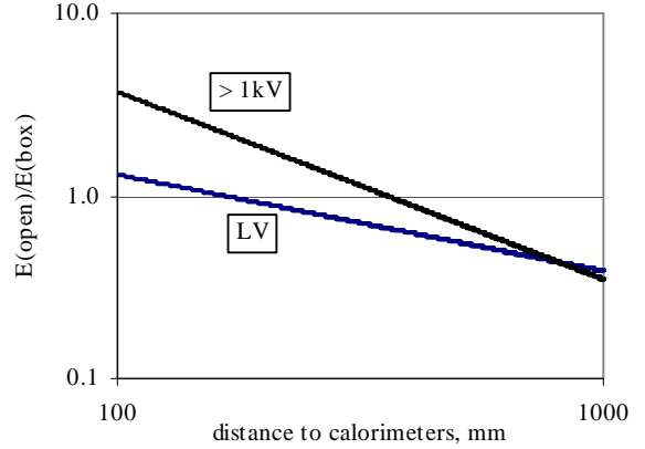
Figure 3. Incident energy ratio using IEEE 1584 equations
