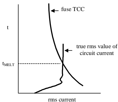
Figure 16. Computation of melting time
