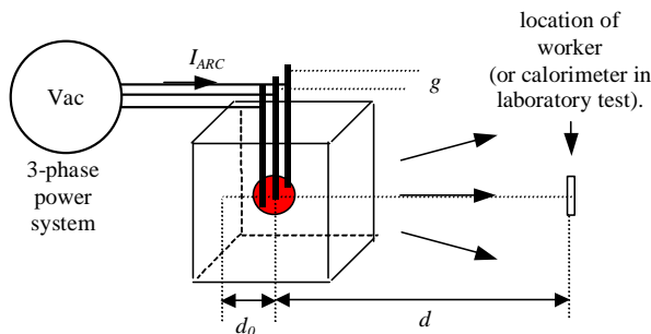
Figure 1. Arc flash in an open box
