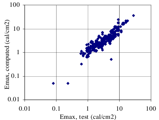
Figure 14. Time domain model prediction compared with test
