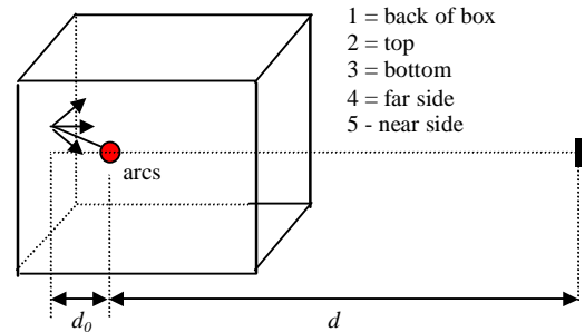
Figure 13. Box geometry for calculation of reflections
