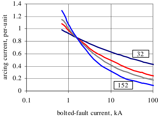
Figure 2. I_{ARC}/I_{BF} calculated from equation (1).
