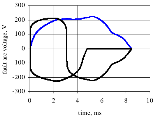
Figure 19. Arcing fault voltages
