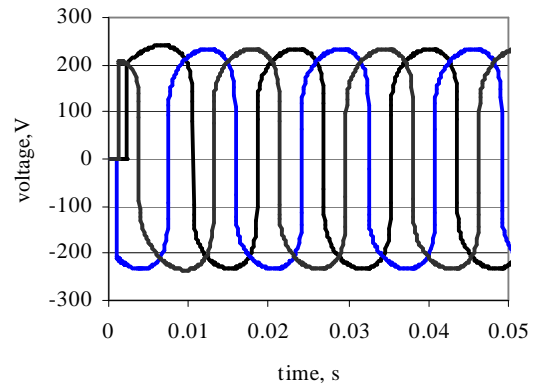
Figure 6. Computed fault arc voltage transients
