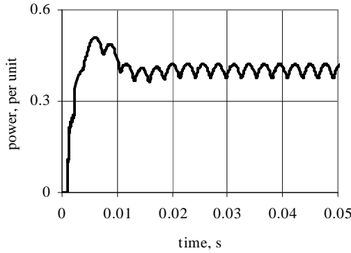
Figure 7. Instantaneous 3-phase power
