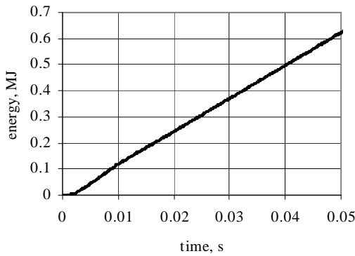
Figure 8. Total arc energy
