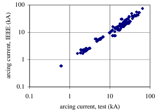
Figure 10. Comparison of predicted and measured arcing current (IEEE 1584 model).
