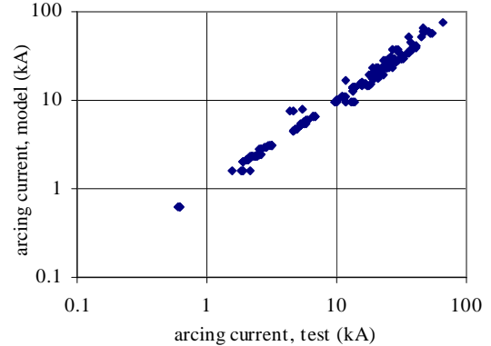
Figure 9. Comparison of predicted and measured arcing current (time-domain model).
