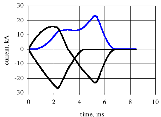
Figure 17. Currents for arcing fault with fuses
