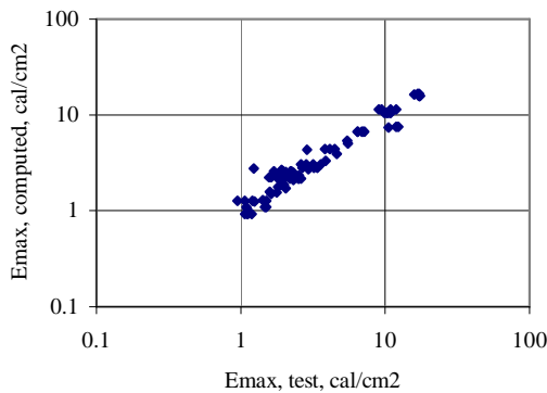
Figure 12. Predicted incident energy density, all open tests
