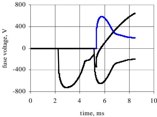
Figure 18. Fuse arc voltages
