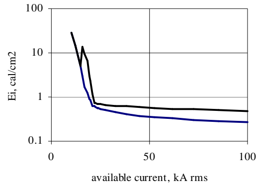
Figure 20. Arc flash characteristic
