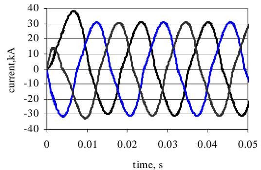
Figure 5. Computed current transients
