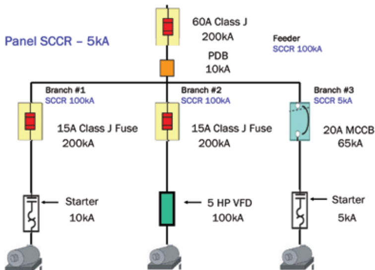
Figure 4: Panel shown with component SCCR adjusted for the current-limiting effects of the 60A Class J fuses in the feeder circuit
